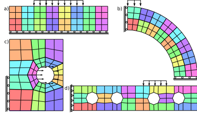
Fig. 5. Coarse grids, boundary conditions and static partition into subdomains for the configurations (a) BLOCK, (b) PIPE, (c) CRACK and (d) STEELFRAME
