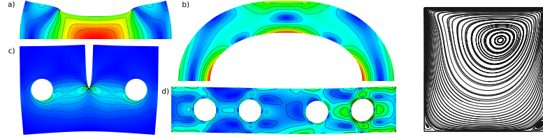
Fig. 6. Computed displacements and von Mises stresses for the CSM configurations, velocity streamline plot for Driven Cavity
