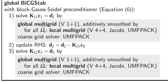
Fig. 3. Our solution scheme for the elasticity equations, scalar solvers are highlighted
