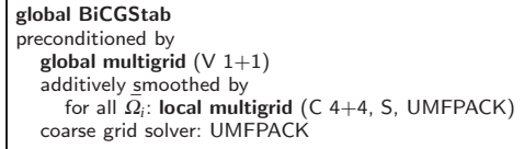
Fig. 2. Illustration of the family of cascaded multigrid solver schemes in FEAST
