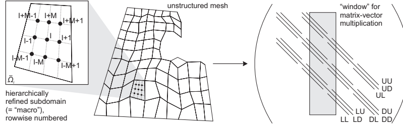
Fig. 1. Grid with logical tensorproduct structure, exemplary one coarse grid cell hierarchically refined. Matrix vector multiplication in SBBLAS operates only on slices of the corresponding FE band matrix
