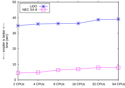
Fig. 7. Weak scalability tests for FEASTSOLID on LiDO and NEC SX-8
