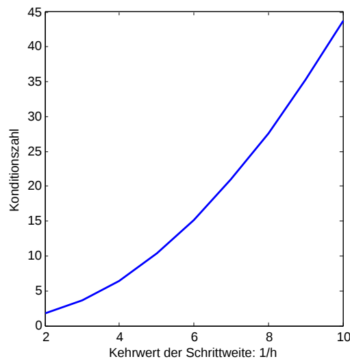
(c) Moderater Referenzwerkstoff: E = \nu = 0.29
