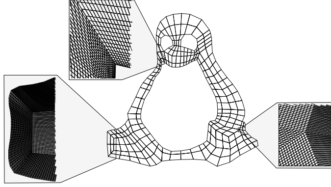
Figure 1: Exemplary TUX geometry. Important features of FEAST’s discretisation approach are highlighted: Globally unstructured, locally structured grids (bottom left, bottom right); anisotropic refinement to, e.g., resolve boundary layers or shock fronts in CFD (microscopic anisotropies, top left); boundary adaption during refinement (bottom left); and coverage of large regions of minor interest with large, regularly refined subdomains (macroscopic feature size variations, bottom right).
