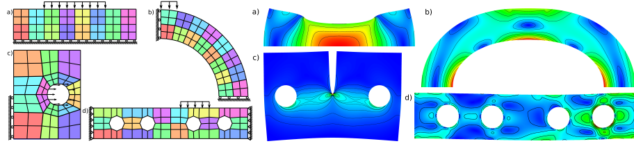
Figure 5: Test problems in linearised elasticity, computed with the GPU-accelerated FEASTSOLID application ((a) BLOCK, (b) PIPE, (c) CRACK, (d) STEELFRAME).
