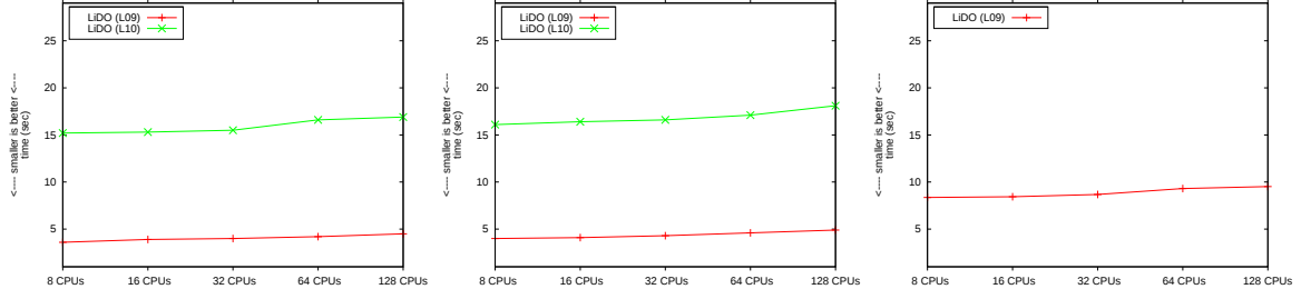
Figure 3: Weak scalability results, normalised to time per iteration.
