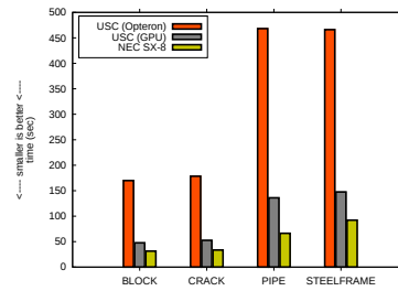
Figure 6: Timing comparison of FEASTSOLID, on USC (with and without GPUs) and NEC SX-8. The longer computation times of the PIPE and STEELFRAME configurations are a consequence of the long and thin structures in conjunction with small Dirichlet boundaries, see Section 4.1.
