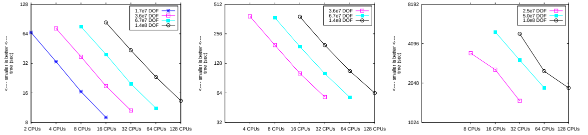
Figure 4: Strong scalability results for the Poisson, FEASTSOLID and FEASTFLOW applications.
