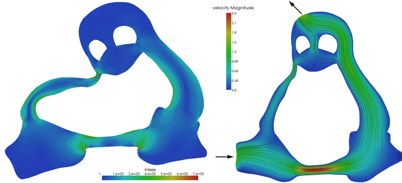
Figure 2: Computed results: Displacements and von Mises stresses for the TUX body under gravity with FEASTSOLID, flow through the TUX body with FEASTFLOW.
