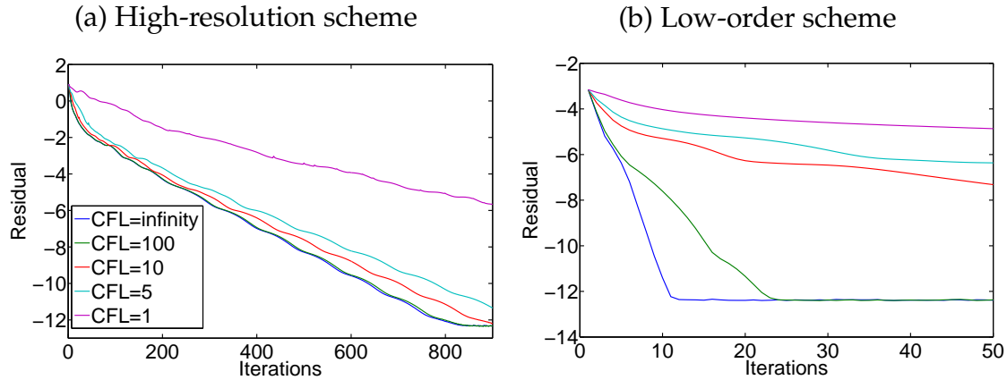
Figure 6: JPL nozzle: Nonlinear convergence history in logarithmic scale for different CFL numbers on mesh level three
