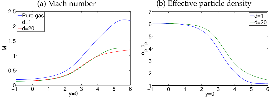
Figure 3: JPL nozzle: Effective particle density in \frac{kg}{m^3} and Mach number at \phi = 0.5
