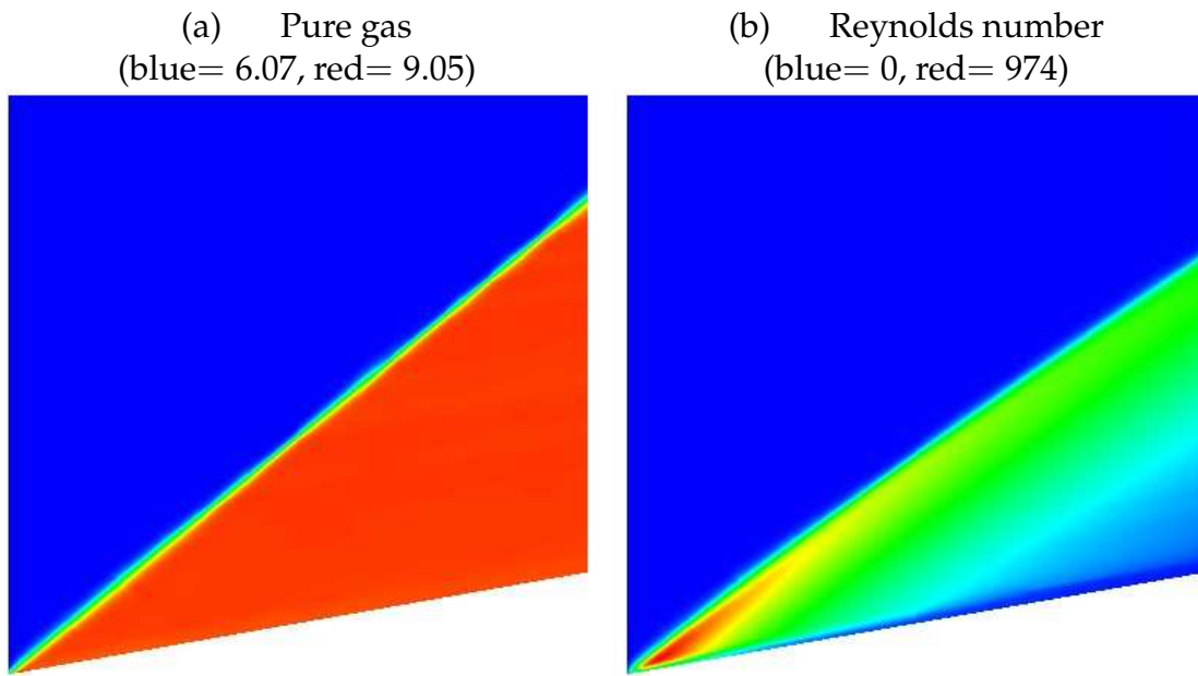
Figure 8: Oblique shock: Pure gas flow density in \frac{kg}{m^3} and Reynolds number with \phi = 0.3 , d = 20\mu m
