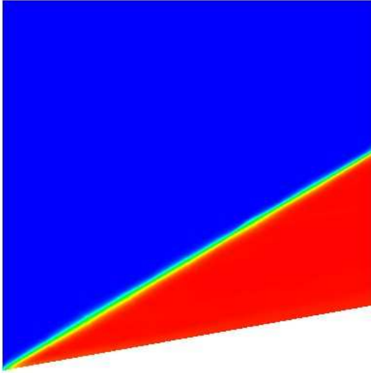
Figure 7: Oblique shock: Effective gas density in \frac{kg}{m^3} for \phi = 0.1, 0.3 and d = 1\mu m, 20\mu m
