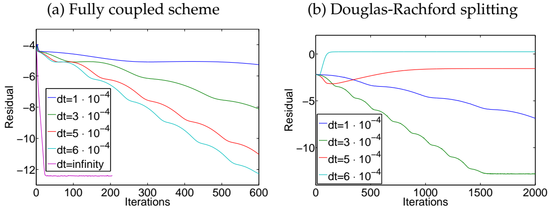
Figure 10: Nonlinear convergence history in logarithmic scale of the low-order schemes for different pseudo time steps on mesh level three
