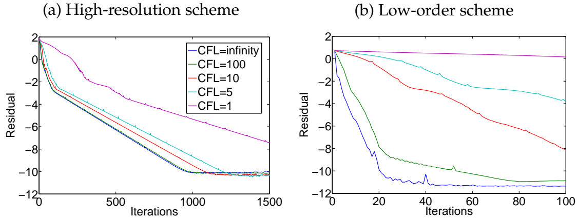
Figure 9: Oblique shock: Nonlinear convergence histories in logarithmic scale
