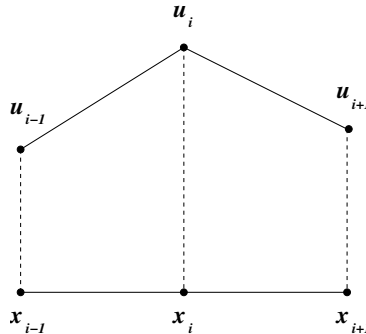
Figure 1. Three-point stencil in one dimension.
