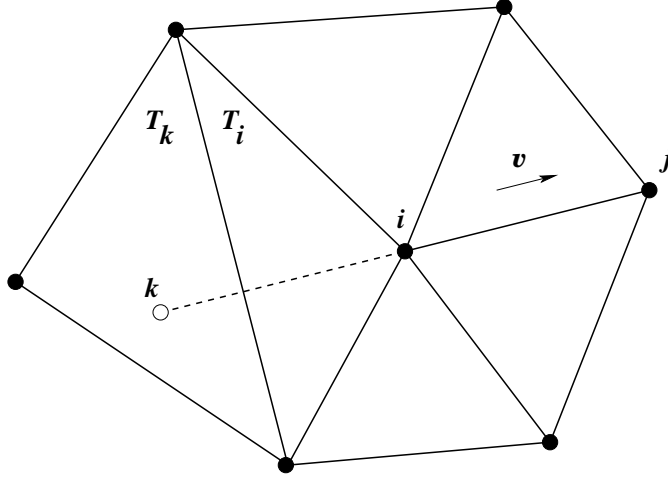
Figure 3. Three-point stencil in two dimensions.
