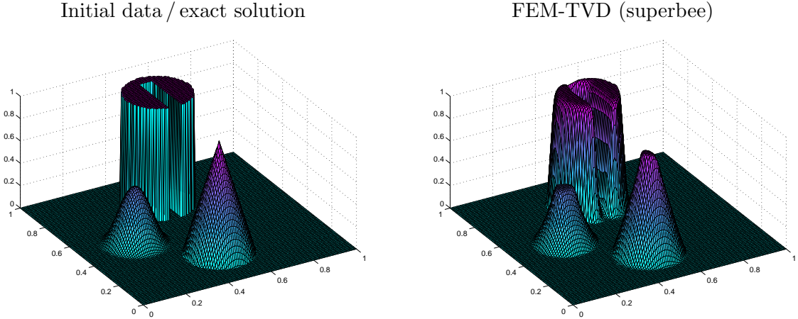
Figure 4. Solid body rotation, 128 \times 128 bilinear elements, t = 2\pi .
