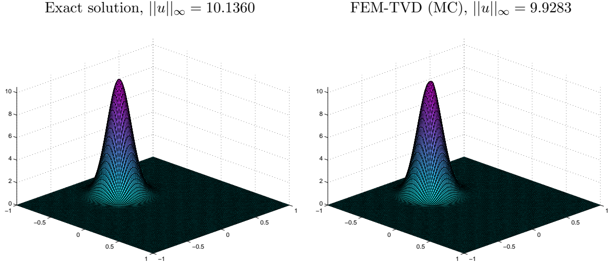
Figure 5. Rotation of a Gaussian hill, 128 \times 128 bilinear elements, t = 2.5\pi .
