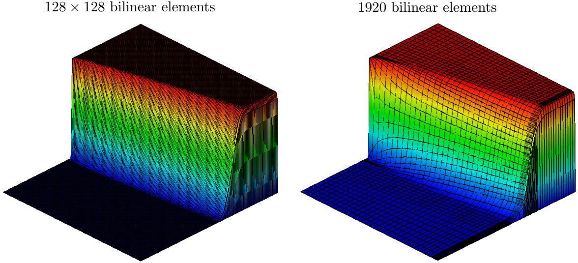
Figure 7. Convection-diffusion, \epsilon = 10^{-3} . FEM-TVD (superbee).
