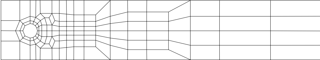
Figure 9. Coarse mesh for the DFG benchmark “Flow around a cylinder”.
