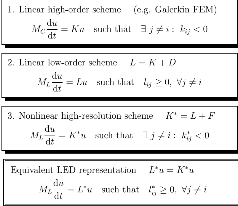
Figure 2. Roadmap of matrix manipulations.
