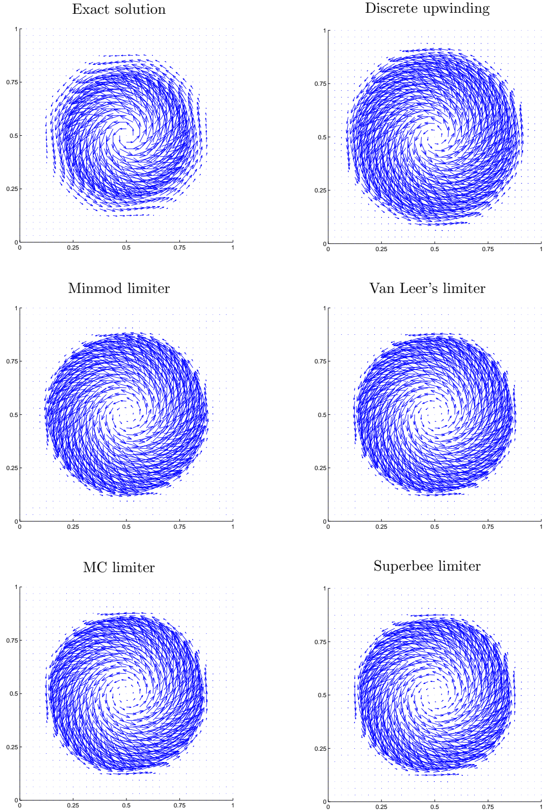
Figure 8. Standing vortex problem. FEM-TVD solution at t = 3 .
