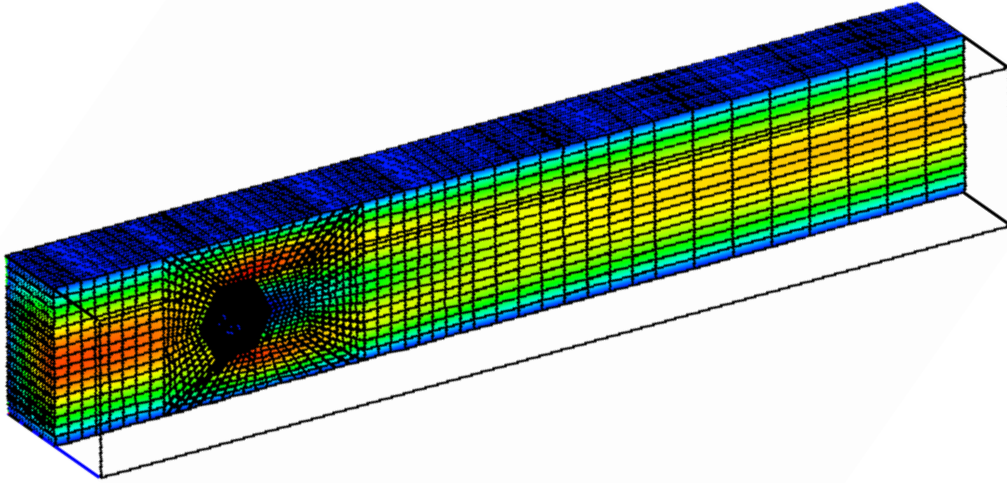
Figure 10. Horizontal velocity. FEM-TVD (MC), 3D projection solver.
