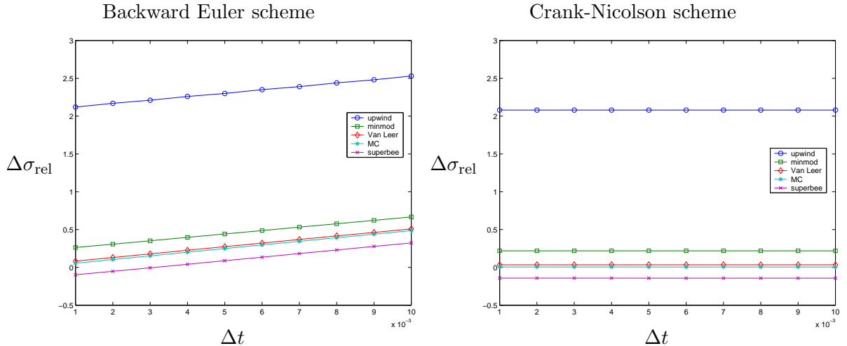
Figure 6. Gaussian hill: relative variance error vs. the time step.
